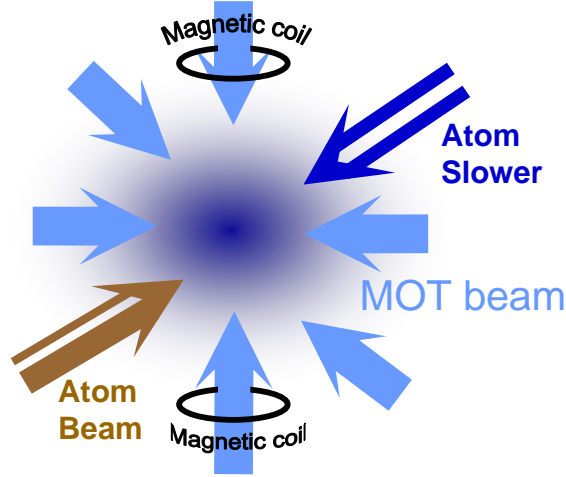
Figure 2.1: Magneto-Optical Trap (MOT). The MOT includes 6 laser beams at 423 nm and the magnetic coils. The coils create a magnetic field that is zero at the trap center.
