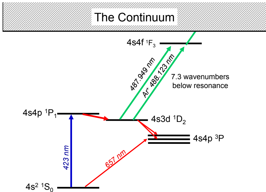
Figure 6.6: Energy Level Scheme for Calcium FORT. Atoms in the ^1D_2 state are trapped. The argon ion laser \lambda = 488 nm excites the atoms and then ionizes from the ^1F_3 state. These ions are subsequently detected in the channeltron
